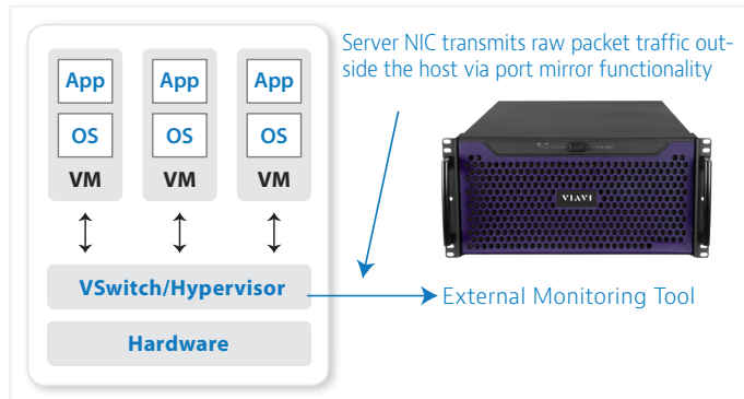
Figure 2. The Outside Virtual Monitoring Model – All analysis performed externally.
