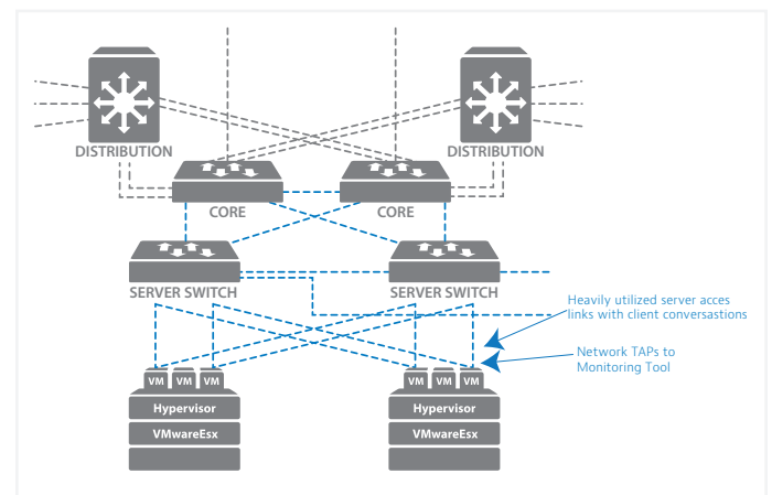
Instrumenting the application server access layer to avoid traffic congestion.
