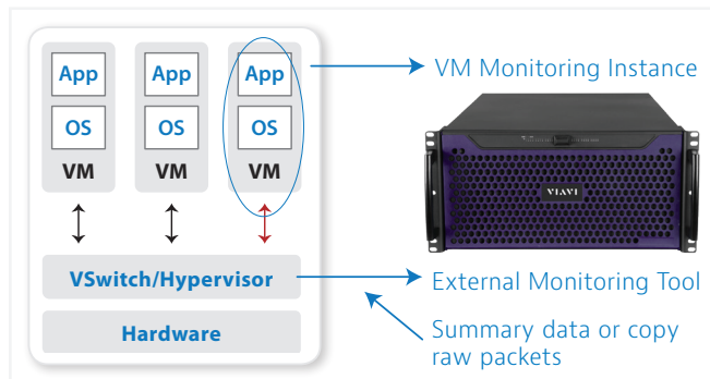
Figure 1. The Inside Virtual Monitoring Model - Virtualized server monitoring using a VM Monitor Instance.
